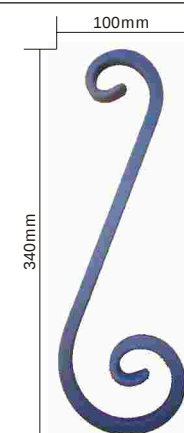
SQUARE BAR
